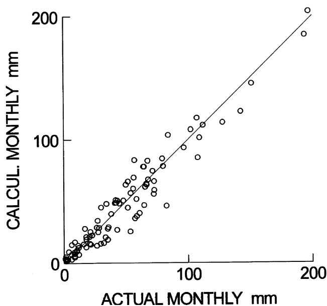
Fig. 10. Boggy Creek catchment—comparison of calculated and actual monthly runoff.
